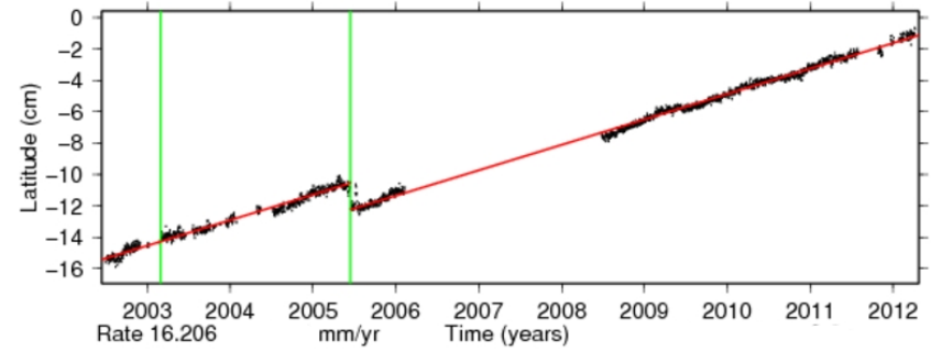
Time series for IQQE.
