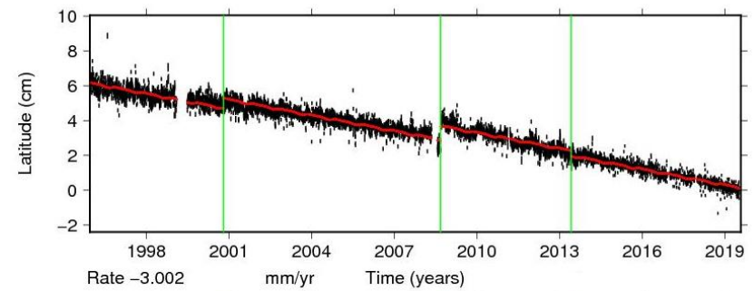
Time series for KERG.
