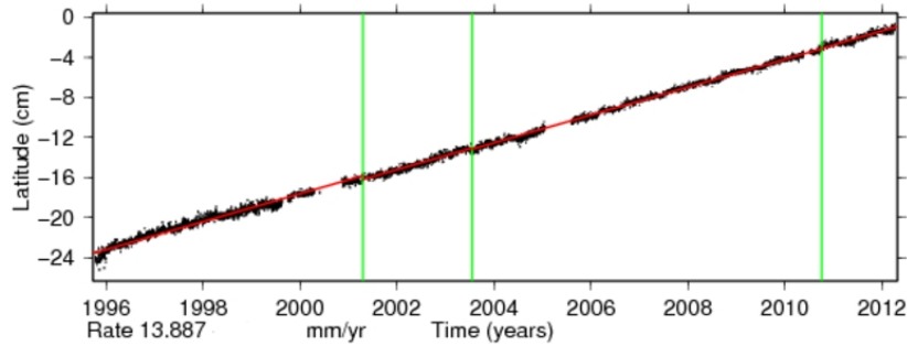
Time series for CRO1.
