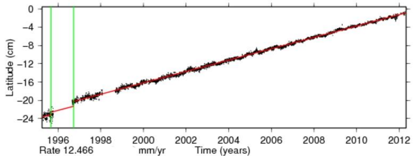
Time series for BRAZ.
