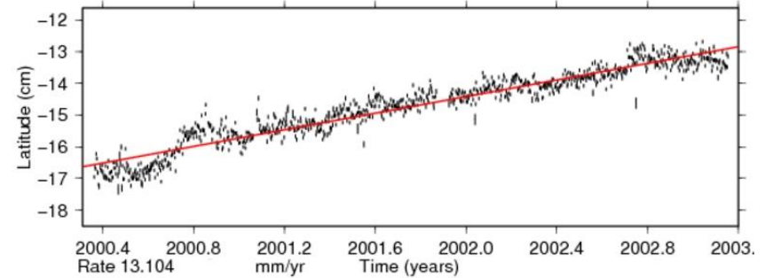
Time series for ESTI.
