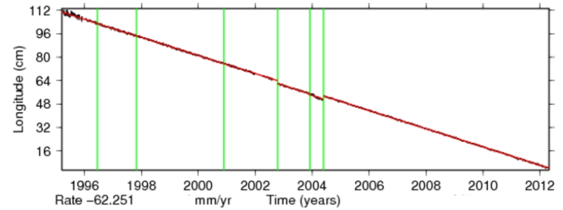
Time series for KERG.
