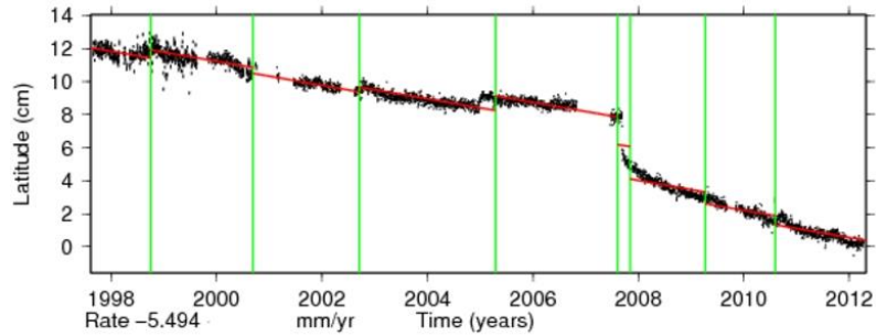
Time series for NTUS.
