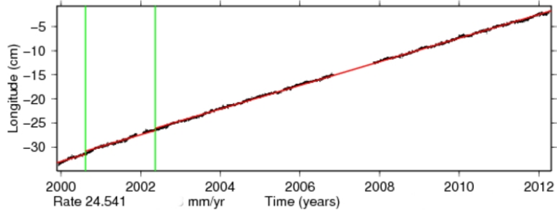
Time series for NTUS.
