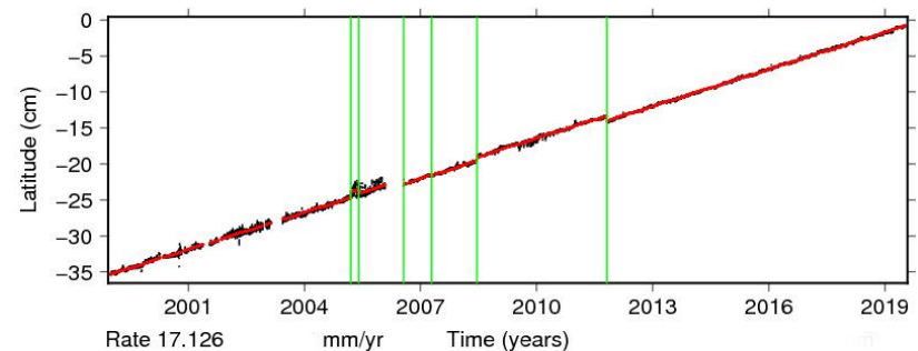
Time series for BRST.
