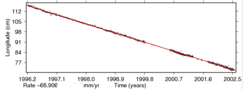
Time series for IQQE.
