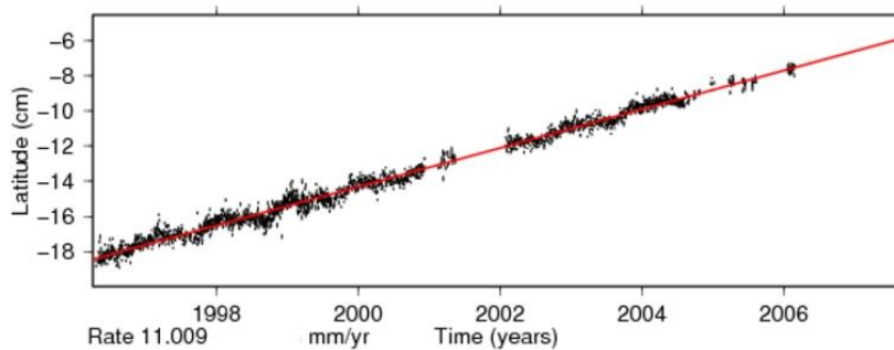
Time series for ASC1.
