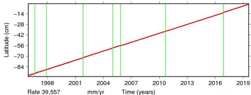
Time series for AUCK.
