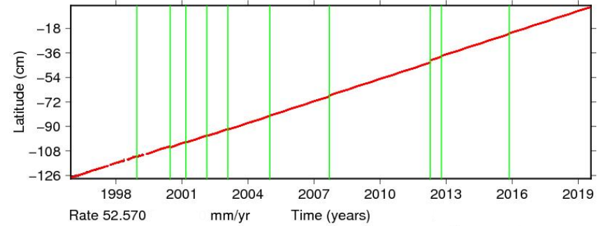
Time series for COCO.
