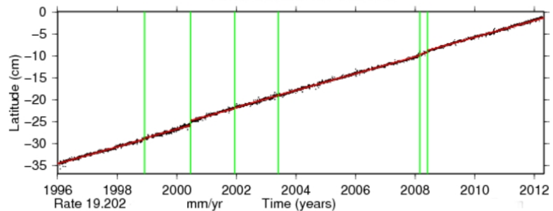
Time series for REYK.
