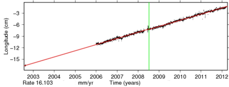
Time series for GUAO.
