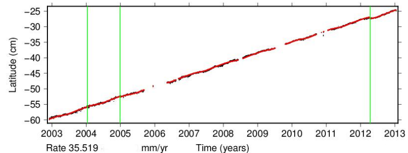
Time series for BAN2.
