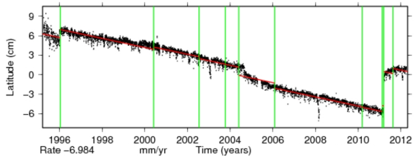
Time series for USUD.
