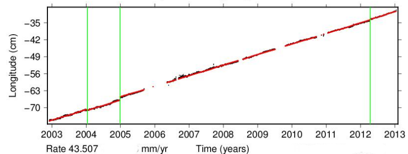
Time series for ASC1.
