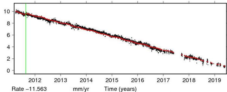
Time series for BJNM.
