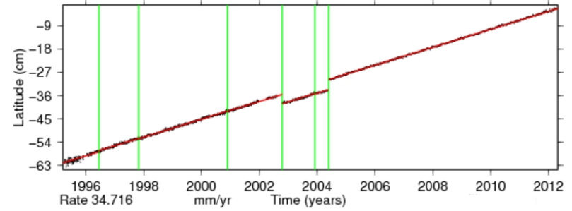
Time series for KOKB.
