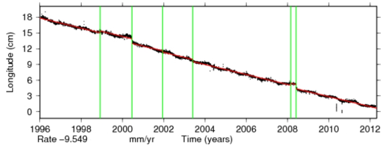
Time series for USUD.
