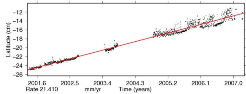
Time series for MSKU.
