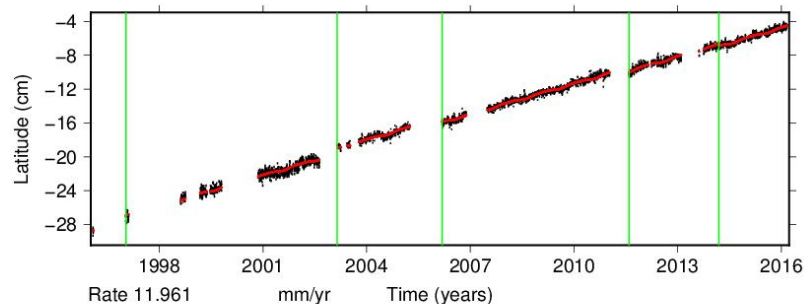
Time series for SEY1.
