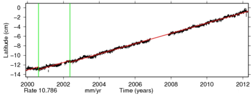
Time series for ISTA.
