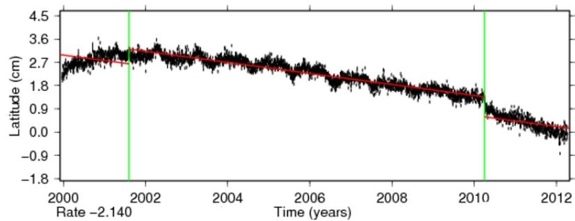
Time series for AGMT.
