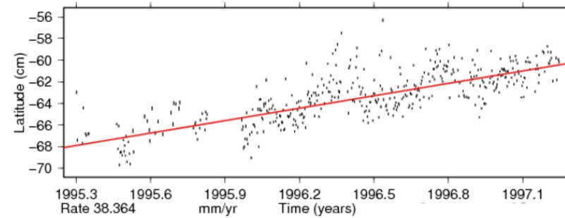
Time series for PAMA.
