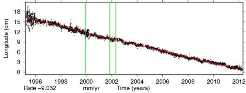
Time series for NJI2.
