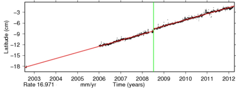
Time series for LPAL.
