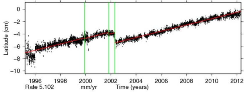
Time series for GUAM.
