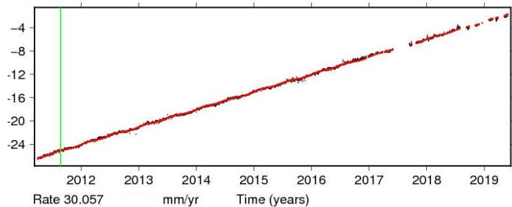
Time series for BRMU.
