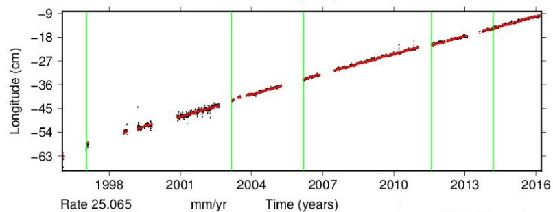
Time series for XIAN.
