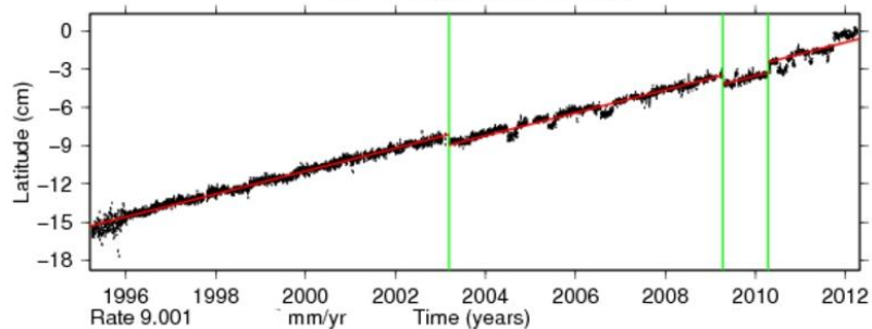
Time series for BRMU.
