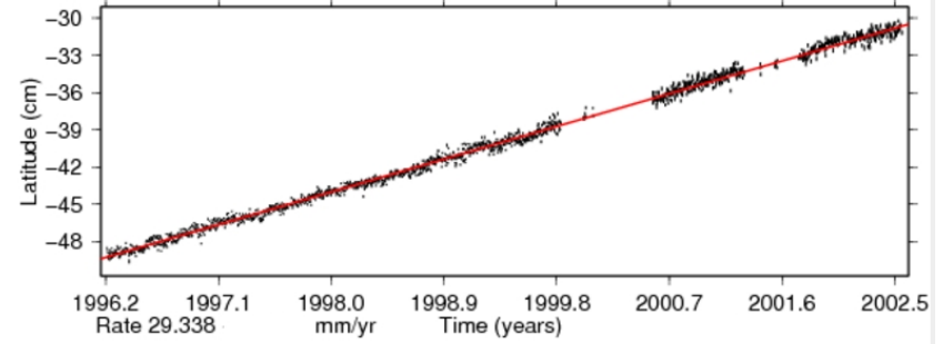
Time series for KWJ1.
