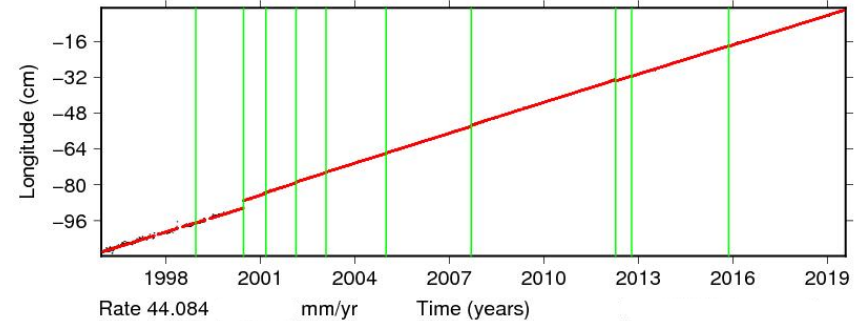
Time series for ESTI.
