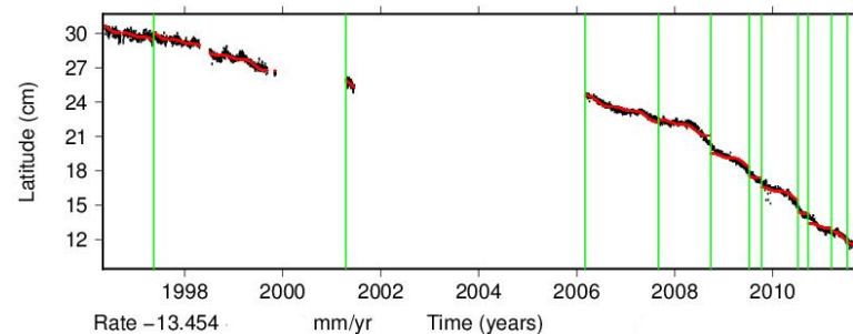
Time series for XIAN.
