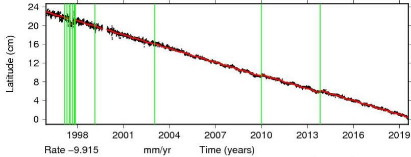
Time series for CAS1.
